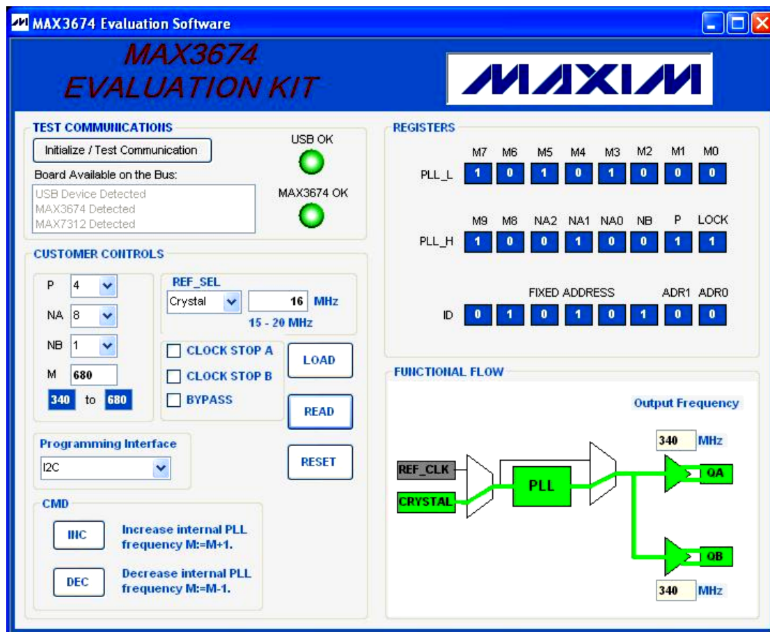
Figure 1. MAX3674 EV Kit Software
