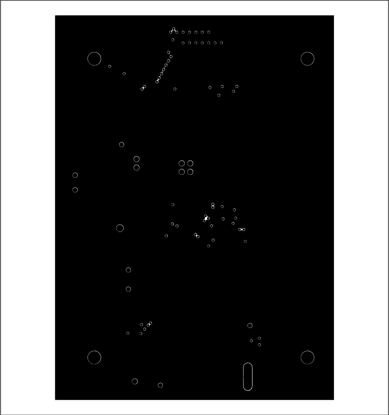
Figure 5. MAX3674 EV Kit PCB Layout—Ground Plane
