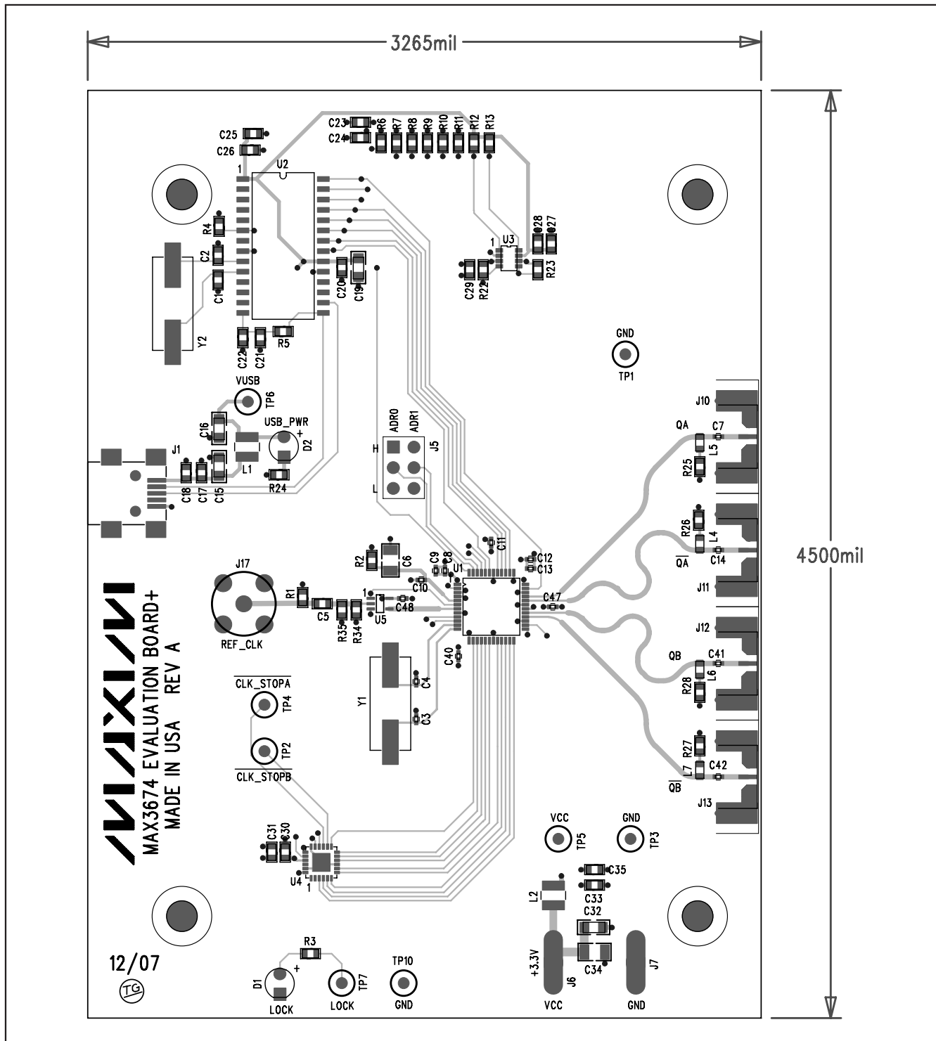
Figure 3. MAX3674 EV Kit Component Placement Guide—Component Side
